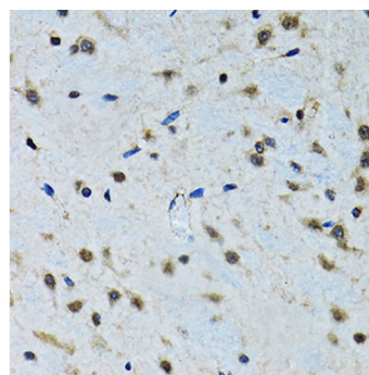
Fig. 2. Immunohistochemistry of paraffin-embedded rat brain using IGF1 antibody at dilution of 1:100 (40x lens).
