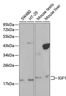
Fig. 1. Western blot analysis of extracts of various cell lines, using IGF1 antibody at 1:1000 dilution. Secondary antibody: HRP-labeled Goat Anti-Rabbit IgG(H+L) (A0208) at 1:1000 dilution. Lysates/proteins: 25µg per lane. Blocking buffer: QuickBlock™ Blocking Buffer (P0231).
